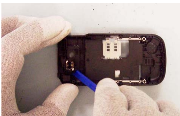
16) Use SS-93 Tool to remove the Earpiece Module.
