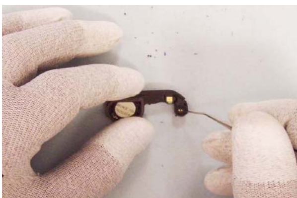
15) Use Pick to remove the Microphone. Avoid bending the spring contacts.
