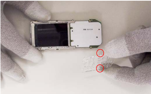
7) Gently release tabs with fingers and remove Keymat Light Guide.
