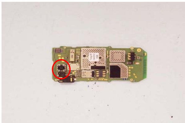
13) Use SS-88 Camera Tool to remove the Camera Module.
