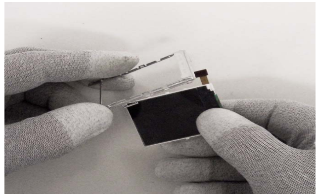
12) Remove the UI Shielding.
