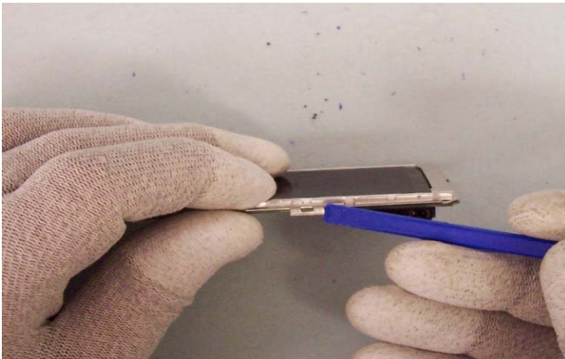
9) Use SS-93 Tool to release LCD tabs
