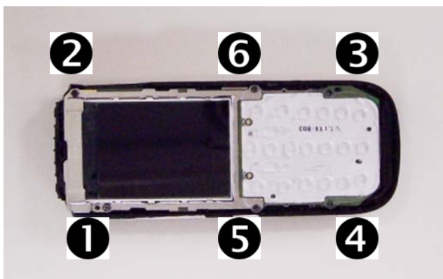
5) Undo the TORX Plus size 4 screws in the order shown.
